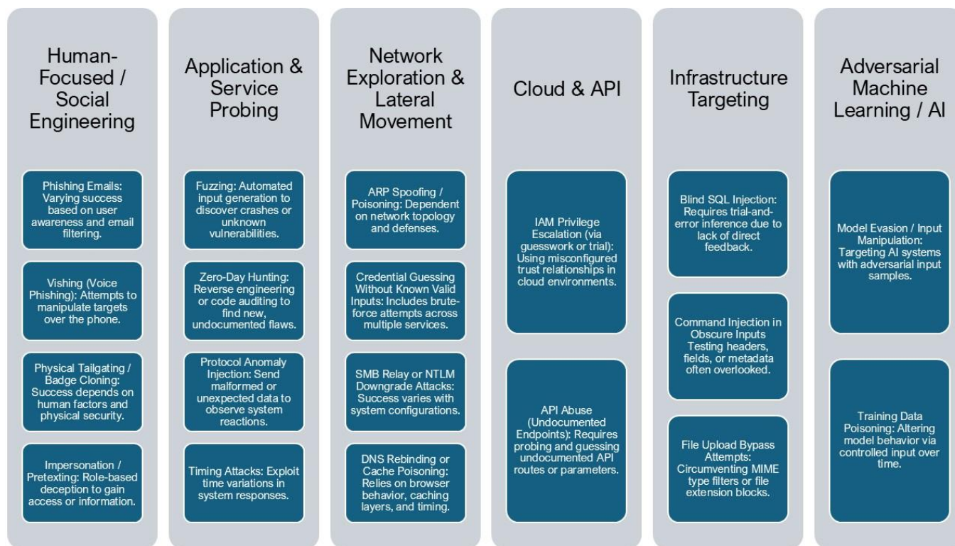
Fig. 1. Non-deterministic penetration testing techniques categorization examples.
